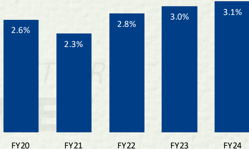
ROA - PBT (%)
