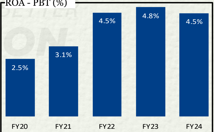
ROA - PBT (%)
