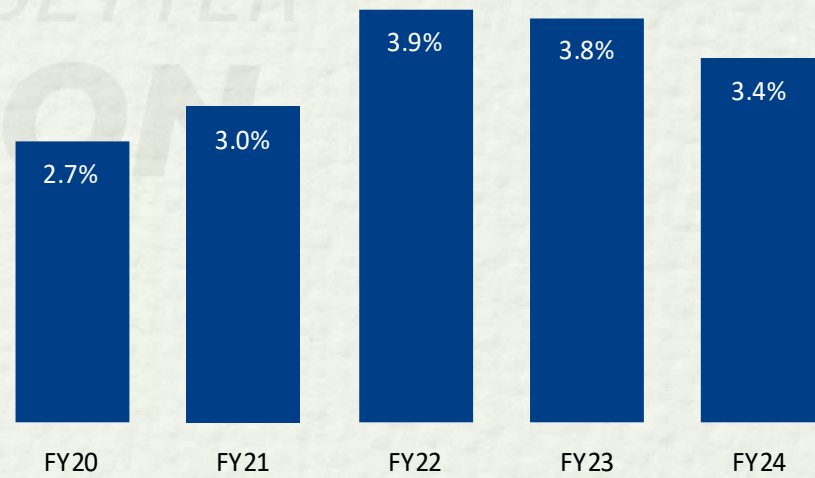
ROA - PBT (%)
